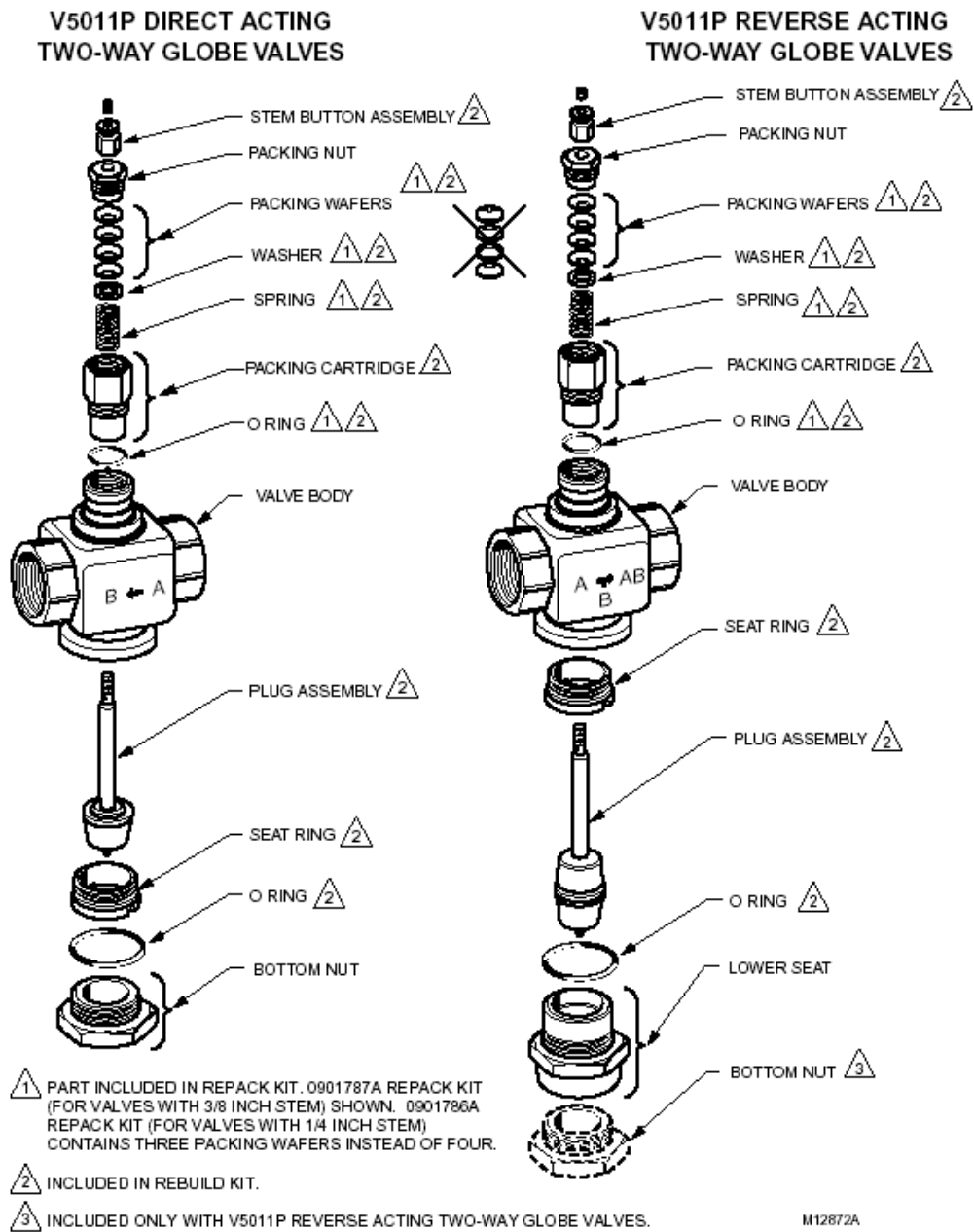
Fig. 5. V5011P replacement parts.
