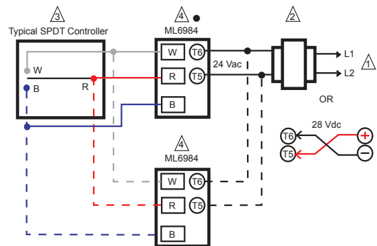
Fig. 9. 3-Wire Control of ML6984 with Electronic Controller.
