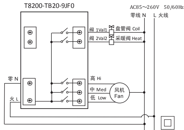
图 4: T8200-TB20-9JF0接线图 Figure 4: Wiring Diagram for T8200-TB20-9JF0
