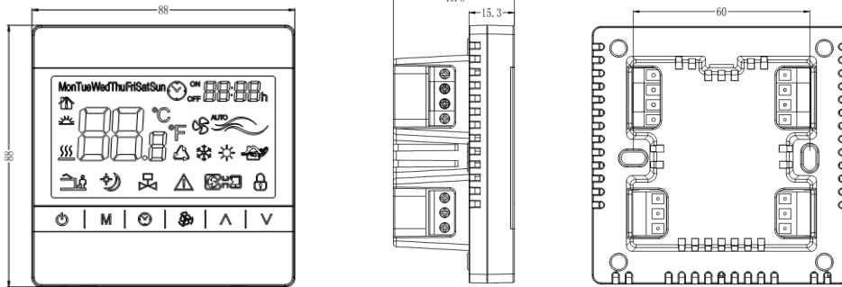
图 2: T8000-TB20-9JF0触摸屏温控器尺寸 (mm) Figure 2: T8000-TB20-9JF0 Touch Screen Thermostat Dimensions (mm)
