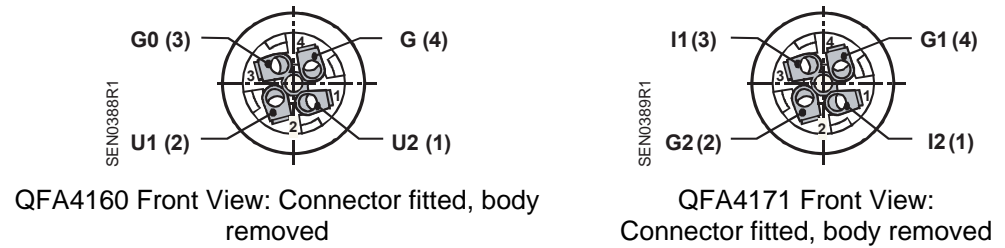
Figure 4. Connectors.
