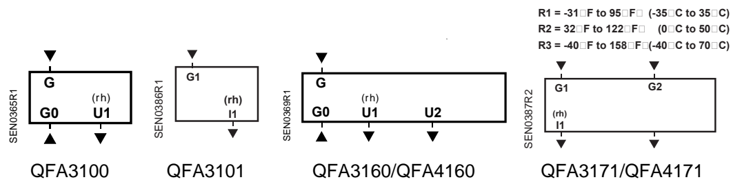
Figure 3. Wiring Terminals.
